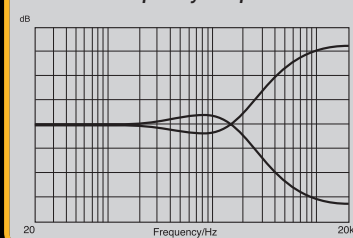
HF Frequency Response
